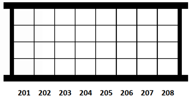
ELEVATION 200 NICHE DIMENSIONS 12 X 12 X 12 MAX URN SIZE 11 X 11 X 11
